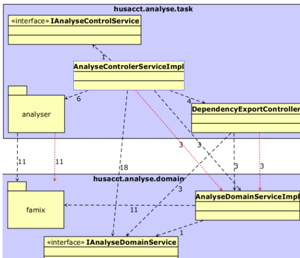
Figure 6. Implemented architecture: Analyse package
