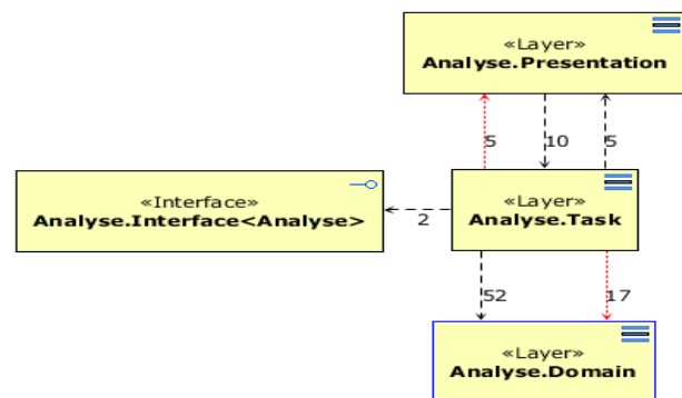
Figure 5. Intended architecture: Analyse component
