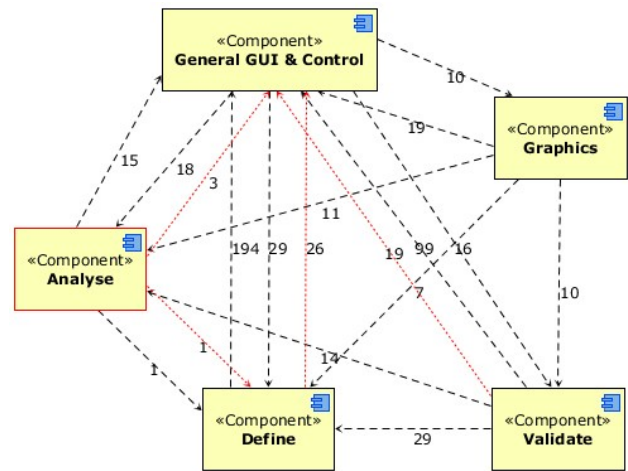
Figure 4. Intended architecture: Top-level components
