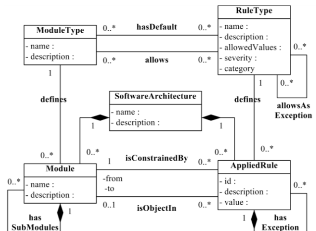
Figure 1. Part of SRMACC metamodel
