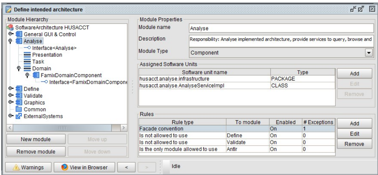
Figure 2. Define intended Architecture, with as case the software architecture of HUSACCT itself
